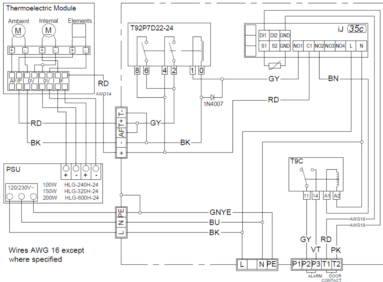
100W / 150W / 200W TE Wiring Diagram 596030797 Rev.b 12.10.2023
